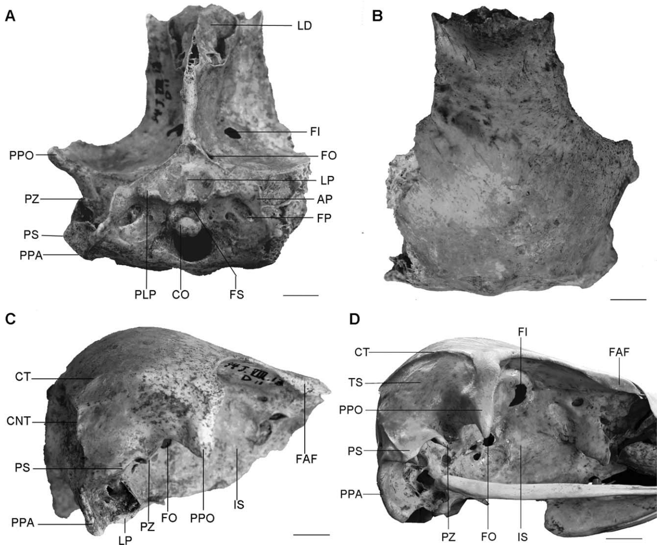
FIGURE 1. Ventral (A), dorsal (B), and lateral (C) views of the cranium of Aegyptius jinniushanensis sp. nov. (94. L. J. A. VIII-13.D-11), and lateral view (D) of the cranium of A. monachus (USNM 18223). Abbreviations: AP, ala parasphenoidalis; CO, condylus occipitalis; CNT, crista nuchalis transversa; CT, crista temporalis; FAF, facies articularis frontonasalis; FI, fonticuli interorbitales; FO, foramen opticum; FP, fossa parabasal; FS, fossa subcondylaris; LD, lamina dorsalis; LP, lamina parasphenoidalis; IS, interorbital septum; PLP, processus lateralis parasphenoidalis; PPA, processus paroccipitalis; PPO, processus postorbitalis; PS, processus suprameaticus; PZ, processus zygomaticus; TS, temporal scar. Scale bars equal 1 cm. (Color figure available online.)
