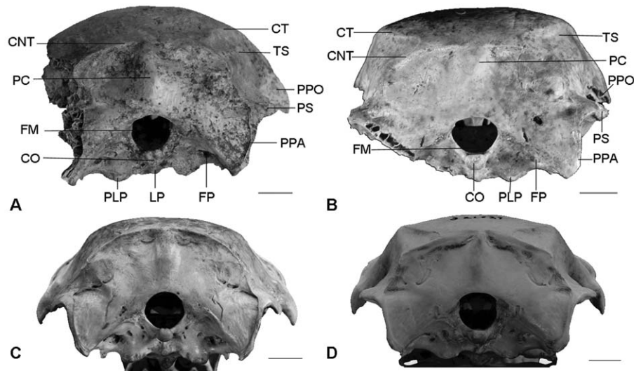
FIGURE 2. Posterior view of crania. A , Aegyptius jinniushanensis sp. nov. (94. L. J. A. VIII-13.D-11); B , Torgos sp. (87. L. J. A. VIII-0: 50); C , Aegyptius monachus (USNM 18223); D , Torgos tracheliotus (USNM 321827). Abbreviations: CNT, crista nuchalis transversa; CO, condylus occipitalis; CT, crista temporalis; FM, foramen magnum; FP, fossa parabasalis; LP, lamina parasphenoidalis; PC, prominentia cerebellaris; PLP, processus lateralis parasphenoidalis; PPA, processus paroccipitalis; PPO, processus postorbitalis; PS, processus suprameaticus; TS, temporal scar. Scale bars equal 1 cm. (Color figure available online.)
